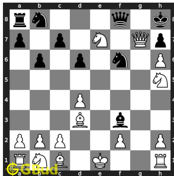
Figure 3: Initial board position of easy chess puzzle 0100
