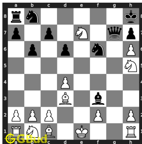
Figure 1: Solve this easy chess puzzle 0100. Mate in 1 move @ https://gbud.in/g3nswm1
